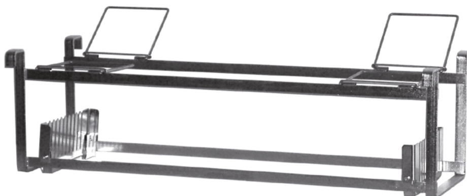
Basket holder KT 70 L with saw blade insert SE 70 L
